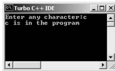
Fig. 16.14 Explaining the usage of switch case statement with break
