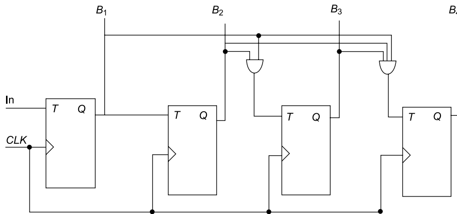
Fig. 9.32 The circuit diagram of synchronous counter
